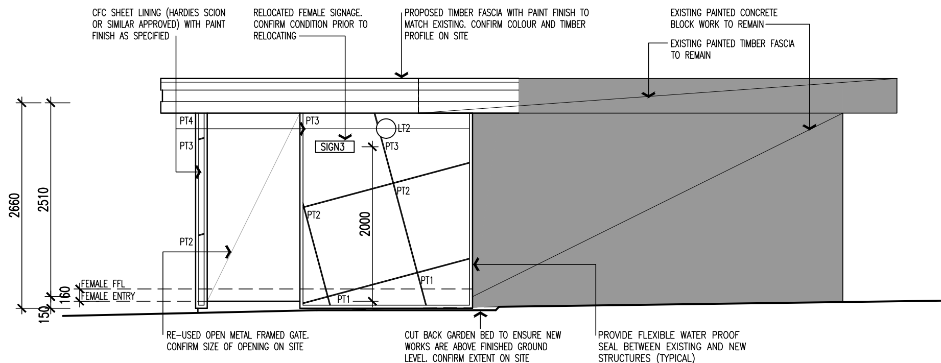
2 SOUTH EAST ELEVATION SCALE: 1:50
