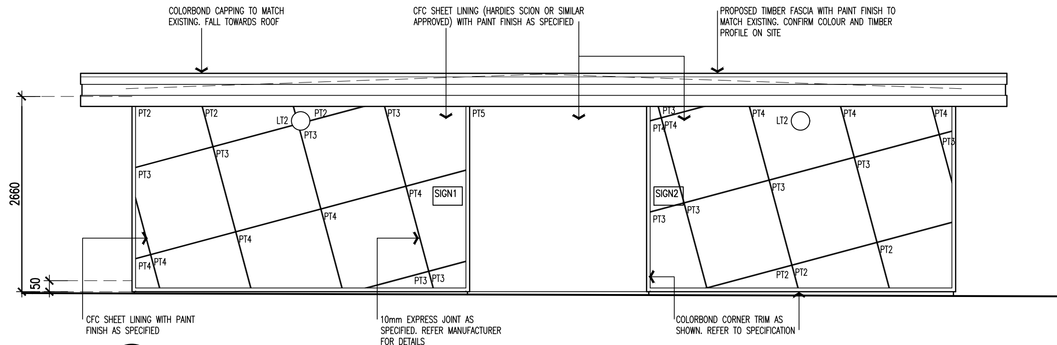
1 SOUTH WEST ELEVATION SCALE: 1:50
